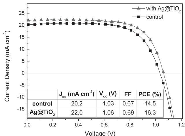
Figure 2. Current density–voltage characteristics for the best control device and optimized \text{Ag@TiO}_2 device. The solar cells were measured via scanning from 1.4 V to short circuit at a scan rate of 0.15 \text{ V s}^{-1} .
